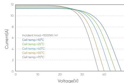
I-V Curve at Different Temperature (385W)
