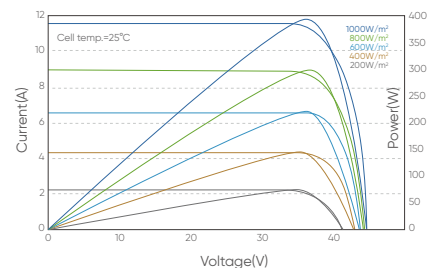
I-V/P-V Curve at Different Temperature (385W)
