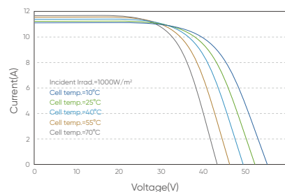
I-V Curve at Different Temperature (465W)
