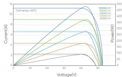
I-V/P-V Curve at Different Temperature (465W)
