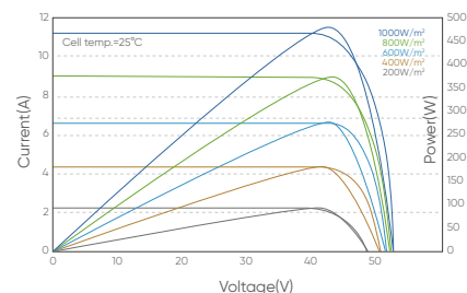
I-V/P-V Curve at Different Temperature (470W)
