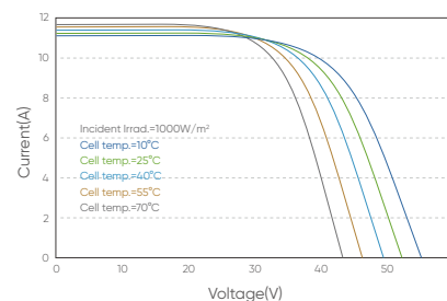
I-V Curve at Different Temperature (470W)
