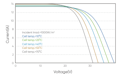
I-V Curve at Different Temperature (425W)
