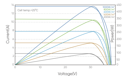
I-V/P-V Curve at Different Temperature (425W)
