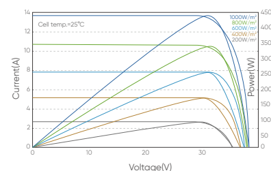
I-V/P-V Curve at Different Temperature (425W)
