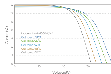
I-V Curve at Different Temperature (425W)
