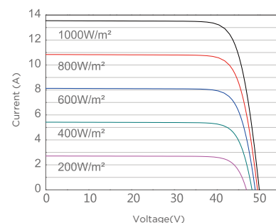
Current-Voltage Curve(MS540M-72H)
