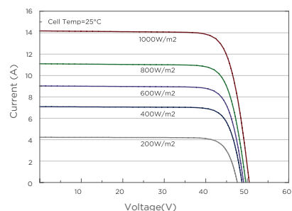
Current-Voltage Curve(MT600M-78H)
