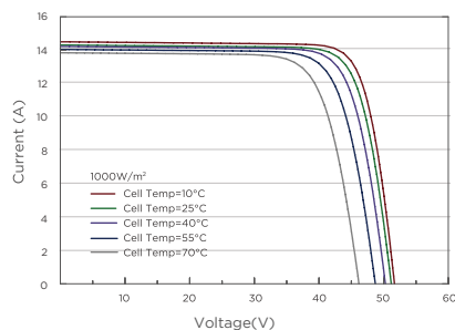
Current-Voltage Curve(MT600M-78H)
