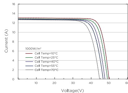
I-V/P-V Curve at Different Temperature (685W)
